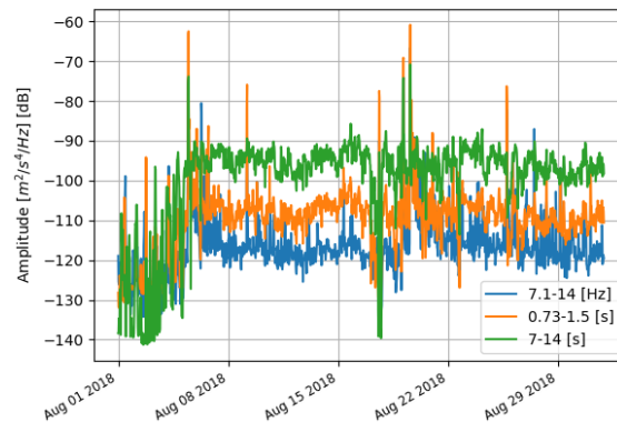
Figure 7. The Spectral probability density value of PLAI
