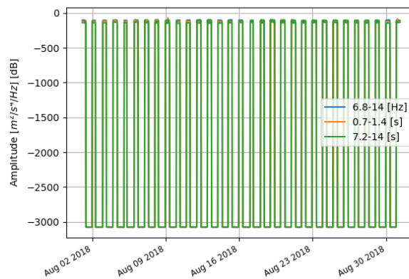
Figure 6. The spectral probability density value of IGBI
