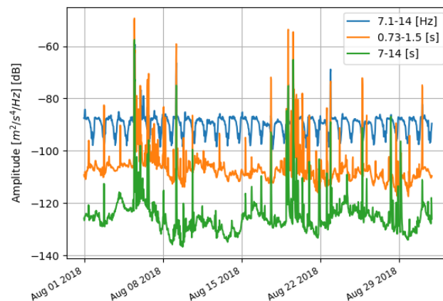
Figure 5. The Spectral Probability Density value of DNP
